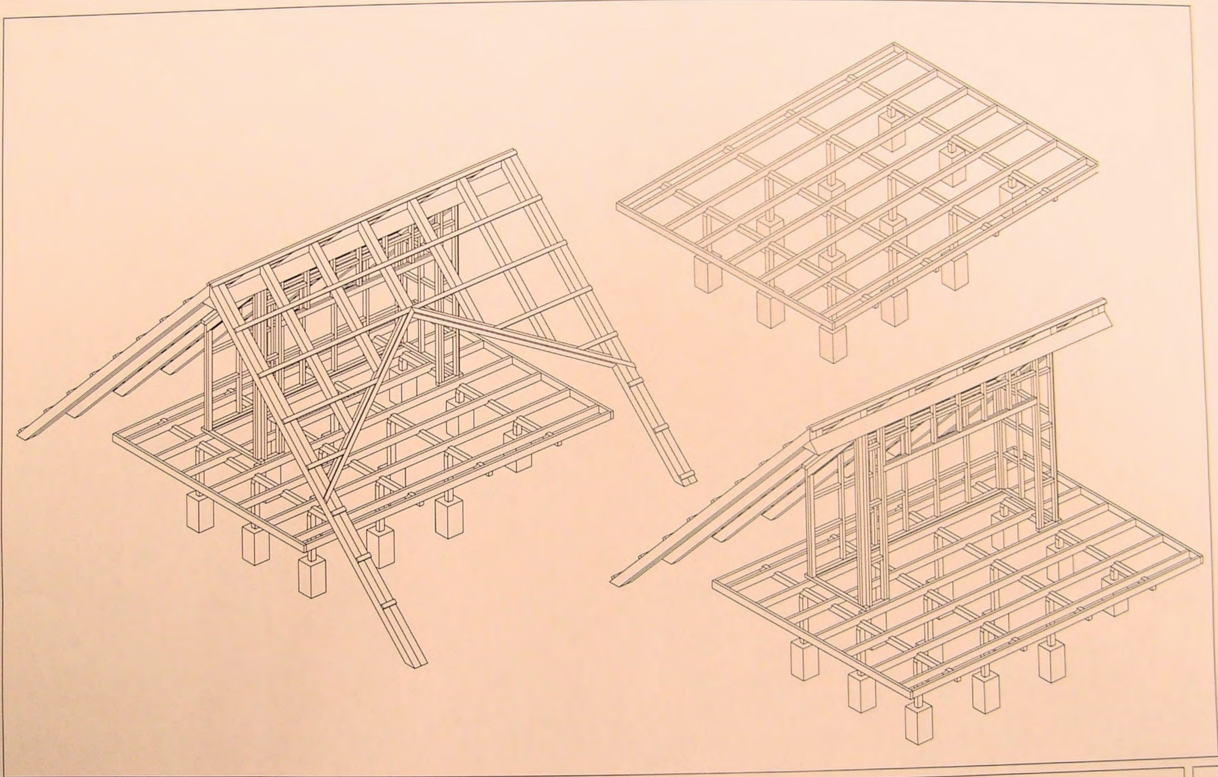
FRAMING ISOMETRIC VIEWS
